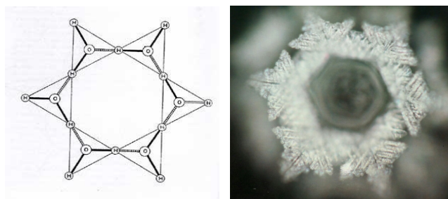
Figure 3. Schematic representation of the cluster of molecules of water that allows for the formation of hexagonal structured water. The angle among such molecules is 120^{\circ} resulting in an hexagonally energized structured. This structure is known as hexagonally energized water 8 .
