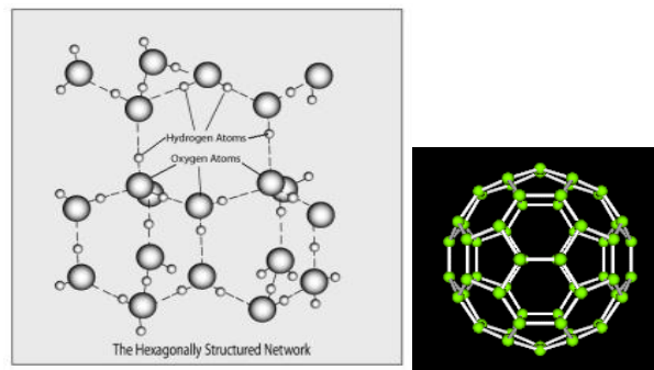
Figure 4. Schematic representation of the water clusters formed with energized hexagonal water. The spherical shape shown is formed with 32 molecules of water, resulting in a truncated structure. To allow for a completely spherical shape another 5 molecules of water are needed, resulting in a cluster made of 37 molecules of water. The resulting structure is highly energized and thus is known as living water, thus bio-water 9 .
